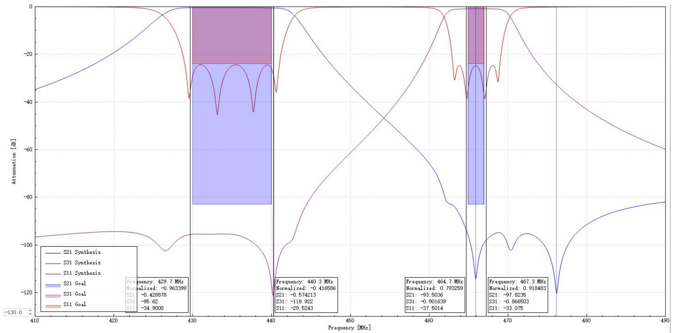
Figure 2 The simulation curve of Duplexer
