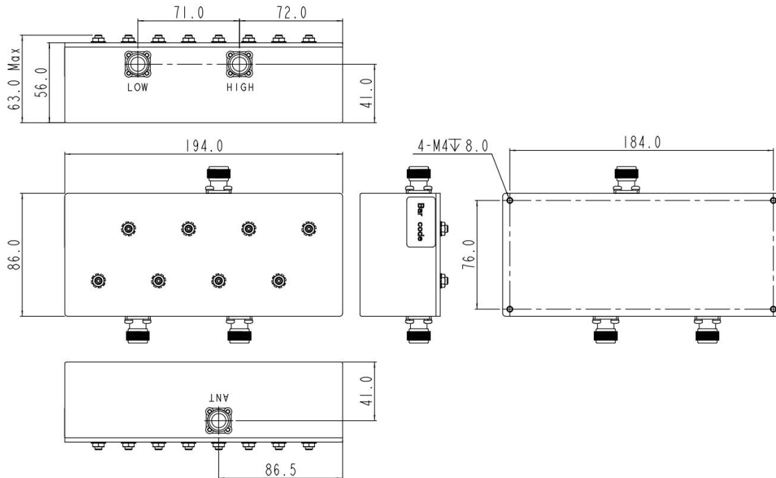
Figure 1 JX-CD2-430M467M-80N front panel layout
